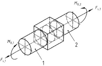
Figure C.3 — Charges appliquées au raccord orthogonal
