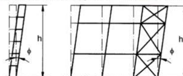
Figure 5.2: Equivalent sway imperfections
