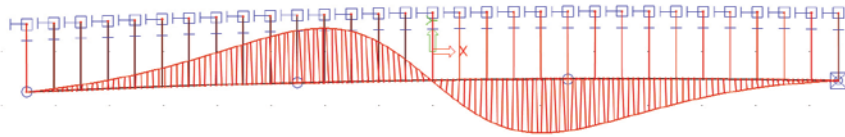
Stability combination S1, Buckling mode 2
