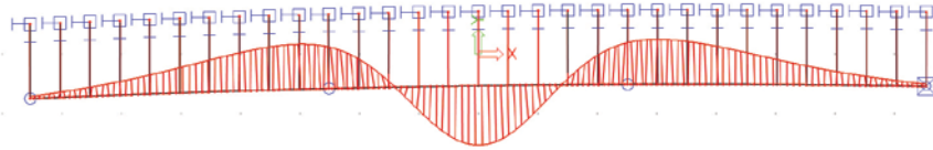
Stability combination S1, Buckling mode 2
